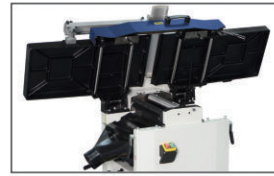
Single Handed table lift, switching from surface planning to thicknessing cannot be easier
